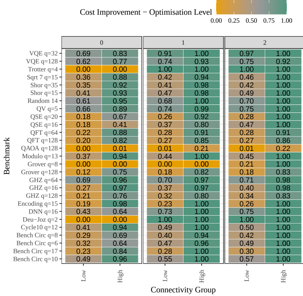
Fig. 17: Cost improvement (see Equations (15), (16), (17)) grouped by optimisation levels (0, 1, 2) and connectivity classes. Optimisation level 1 often performs comparably to level 2, suggesting it is the more efficient choice when compile time is considered. Performance improves significantly with connectivity, reinforcing its dominant influence.
