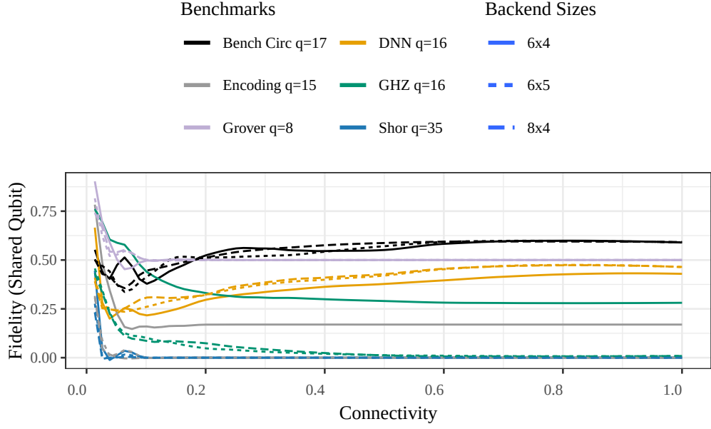
Fig. 8: Impact of back-end size fidelity as a function of connectivity across benchmarks for crosstalk version shared qubit.
