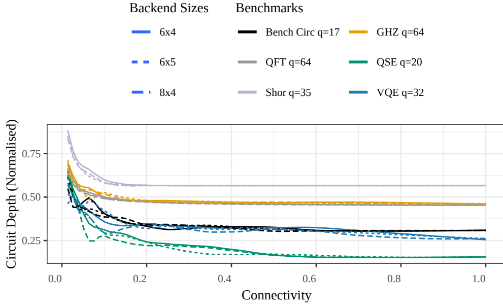
Fig. 10: Impact of back-end size on normalised circuit depth as a function of connectivity across benchmarks.
