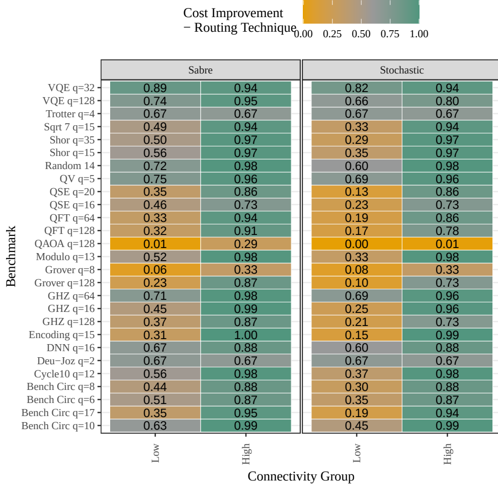
Fig. 16: Cost improvement (see Equations (15), (16), (17)) for routing techniques (SABRE, Stochastic), grouped by low and high connectivity. SABRE outperforms Stochastic in almost every case.
