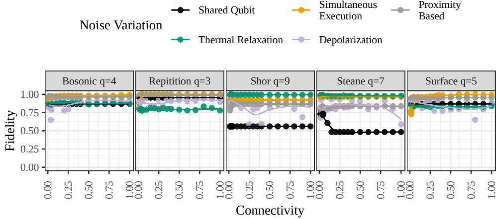
Fig. 3: Extension of Figure 2 with error correcting codes.
