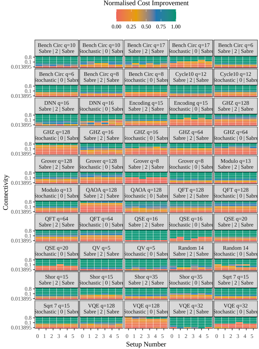
Fig. 18: Cost improvement (see Equations 15 16, 17) vs. connectivity across benchmarks and compilation setups. Improvements are measured relative to the baseline configuration with no additional improvements.
