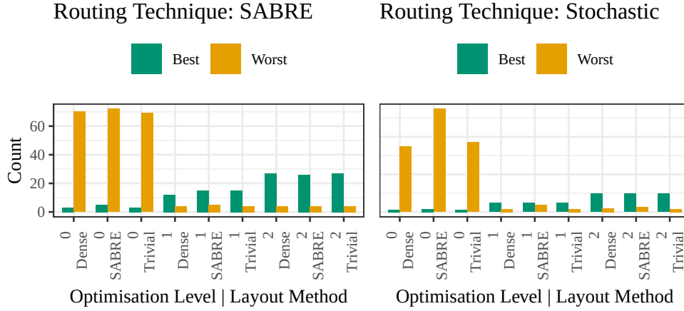
Fig. 11: Frequency of best and worst-performing combinations, based on cost improvement, evaluated across qubit routing technique, layout method, and optimisation level over all benchmarks and connectivity densities
