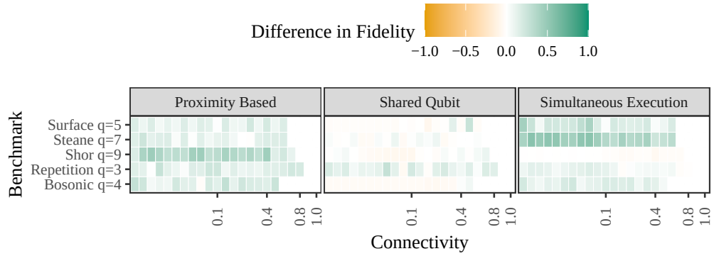
Fig. 7: Extension of Figure 6 with error correcting codes.
