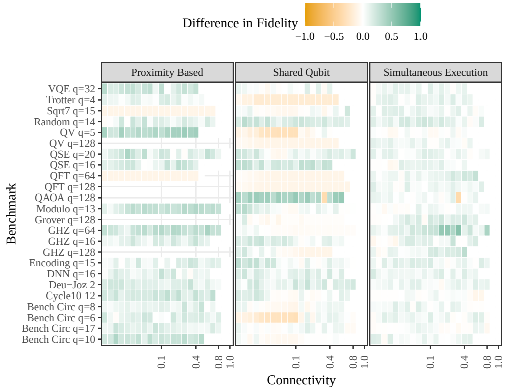
Fig. 6: Difference in fidelity between heavy-hex and the grid-like topology of the Sycamore chip across benchmarks and connectivity.
