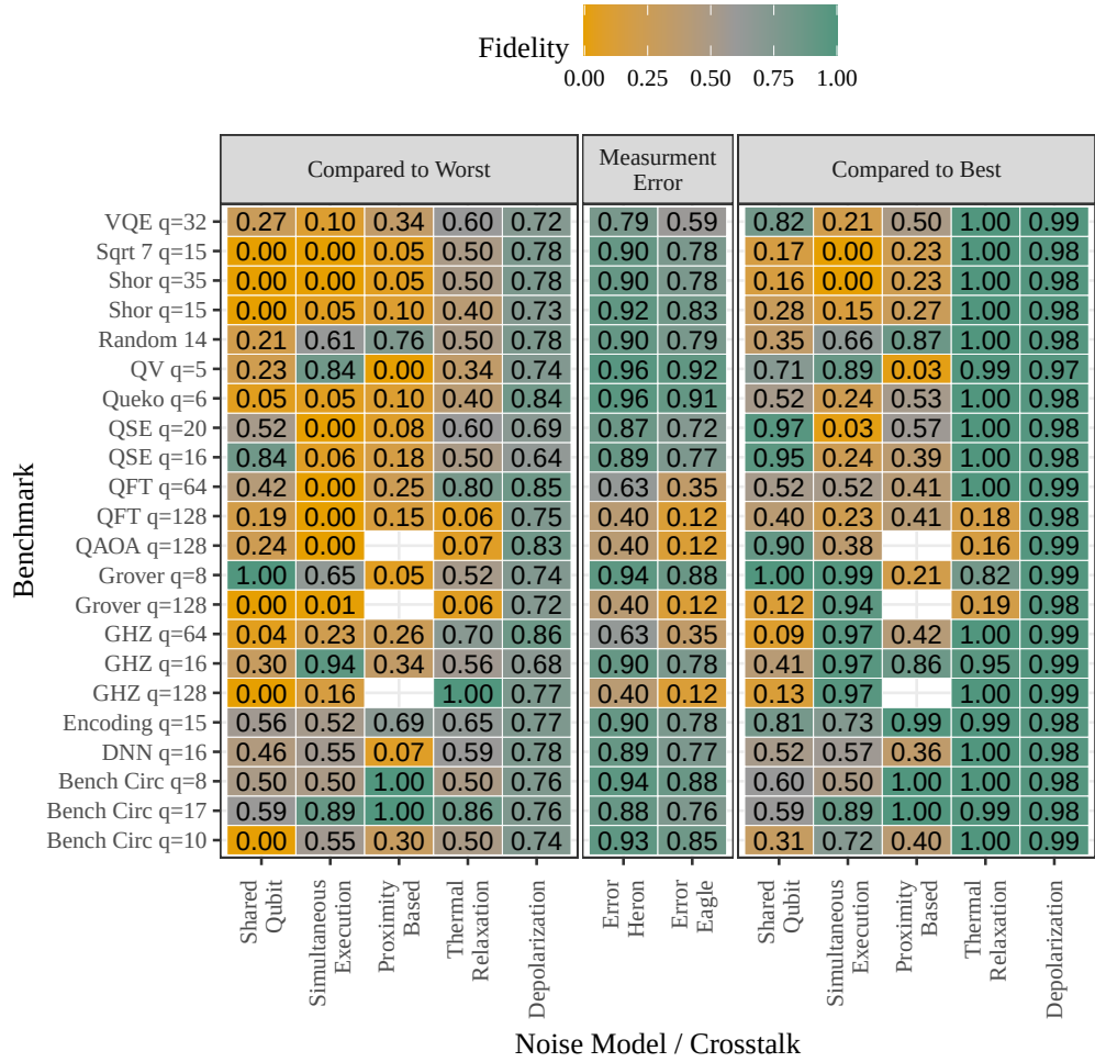
Fig. 5: Fidelity comparison for all benchmarks under different noise models. For each benchmark, we show the lowest (worst) and highest (best) fidelities obtained across all connectivity values and crosstalk/noise models evaluated. These values are then compared to the fidelities achieved under measurement error for the IBM Heron and Eagle processors. The columns "Compared to Worst" and "Compared to Best" show how measurement error performance relates to the fidelities observed in our detailed crosstalk and noise model calculations.
