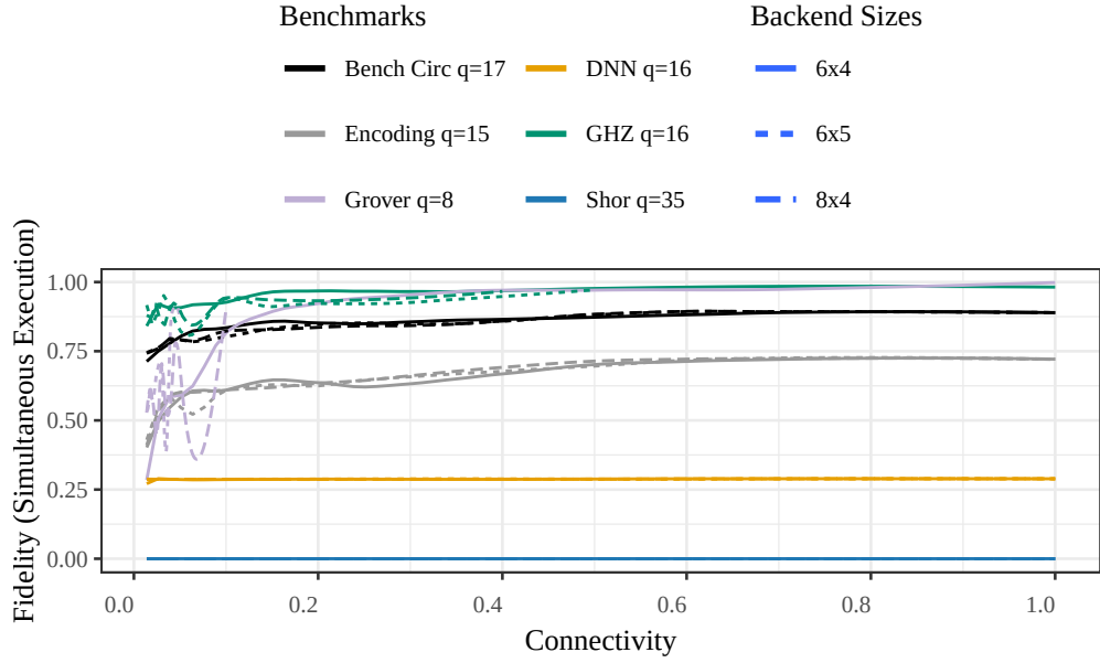
Fig. 9: Impact of back-end size fidelity as a function of connectivity across benchmarks for crosstalk version simultaneous execution.
