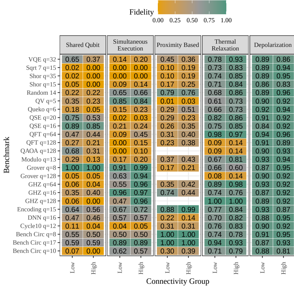
Fig. 4: Table view summarising the average fidelity of various quantum benchmarks under different noise models across two connectivity groups: Low ( \leq 0.25 ) and High ( \geq 0.3 ). The x-axis represents the connectivity group, and the y-axis lists the benchmarks. Each facet column corresponds to a different noise model: Shared Qubit, Simultaneous Execution, Proximity Based, Thermal Relaxation, and Depolarization. Cell values show the average fidelity rounded to two decimal places. For Shared Qubit, fidelities often decrease with higher connectivity, while for all other noise models—including Thermal Relaxation and Depolarization—fidelity typically improves as connectivity increases.
