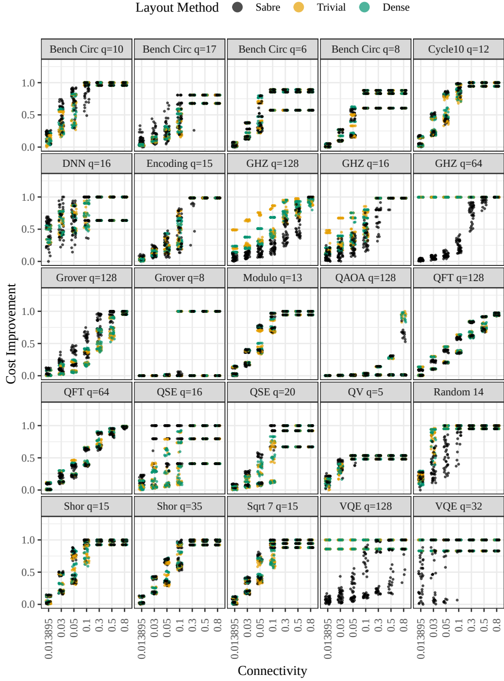
Fig. 12: Cost improvement (see Equations (15) (16), (17)) vs. connectivity across benchmarks for three layout methods.
