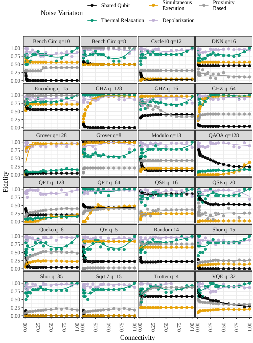
Fig. 2: Illustration of fidelity vs. connectivity across benchmarks as facets comparing three crosstalk models, thermal relaxation, and depolarisation noise for the heavy-hex back-end topology.
