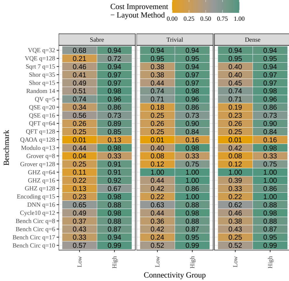
Fig. 15: Cost improvement (see Equations (15), (16), (17)) for different layout methods (SABRE, Trivial, Dense), grouped by low ( \leq 0.25 ) and high ( \geq 0.3 ) connectivity. The figure emphasises the benefit of high connectivity for nearly all benchmarks.
