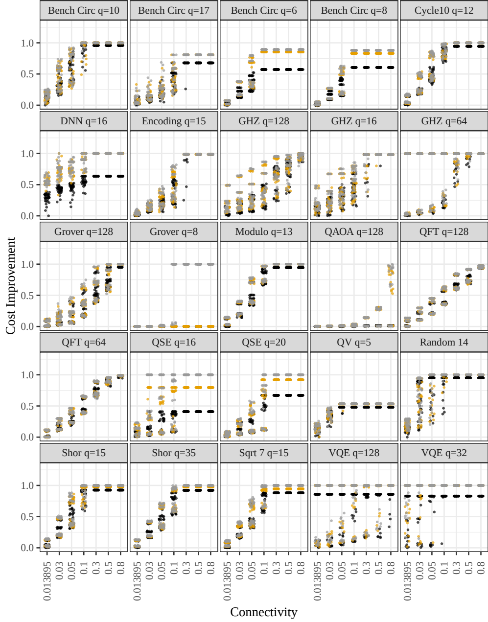
Fig. 14: Illustration of cost improvement as defined in Equations (15) (16), (17) vs. connectivity across benchmarks as facets comparing three optimisation levels.
