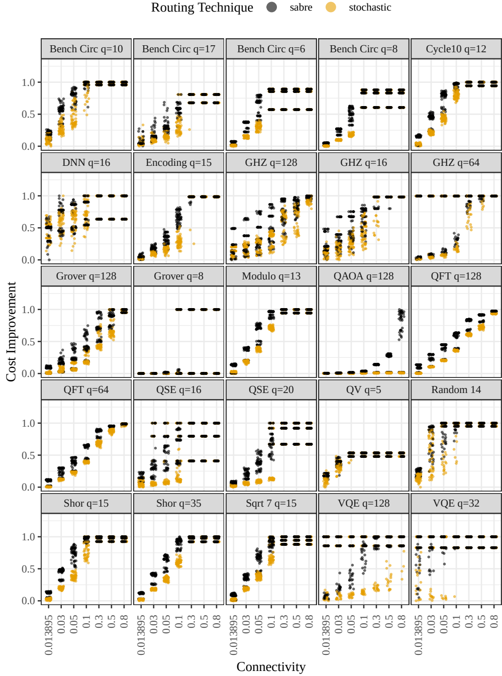
Fig. 13: Illustration of cost improvement as defined in Equations (15) (16), (17) vs. connectivity across benchmarks as facets comparing two routing techniques.
